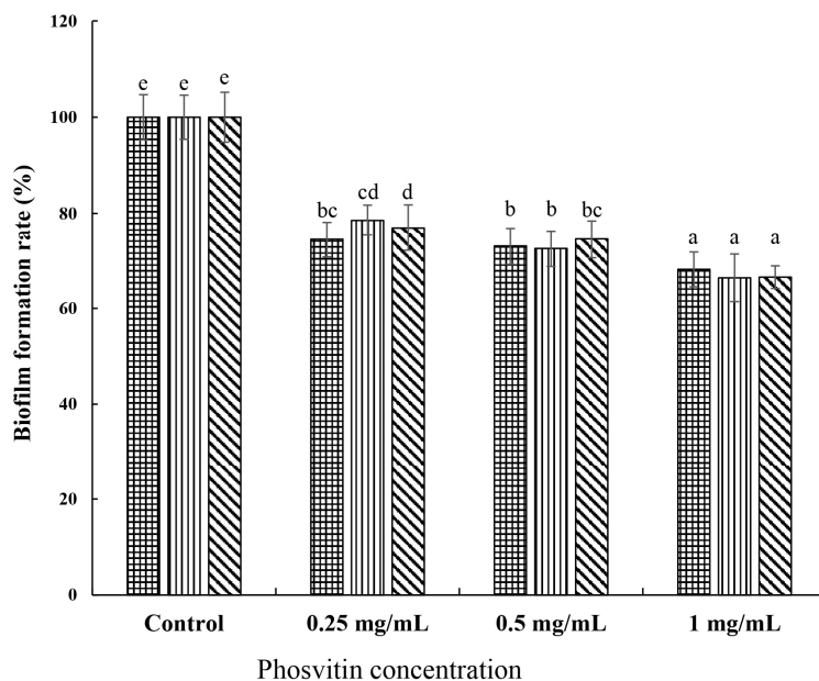
Fig. 2. Effects of phosvitin on preformed biofilm against Streptococcus mutans . ■, S. mutans KCTC 5124, ▨, S. mutans KCTC 5458, and ▩, S. mutans KCTC 5316. Values are expressed as the mean±SD. a-e Different letters among samples indicate significant differences (p<0.05). Control, non-treated group.
