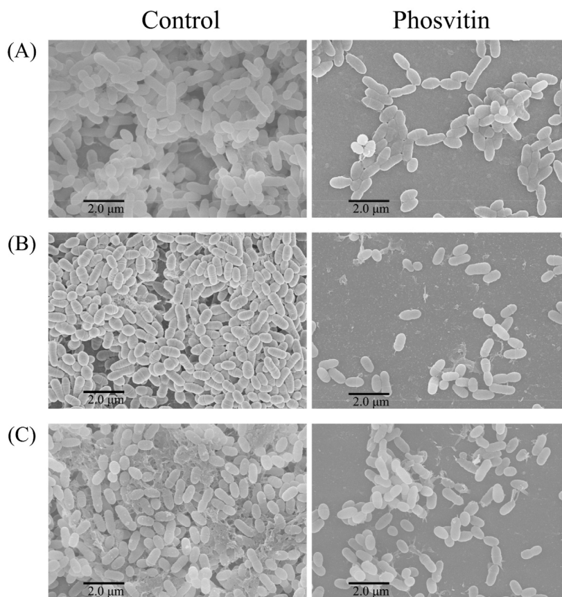
Fig. 6. Scanning electron micrographs of Streptococcus mutans biofilms on glass coverslips treatment with phosvitin 1 mg/mL. (A) S. mutans KCTC 5124, (B) S. mutans KCTC 5458 and (C) S. mutans KCTC 5316. Control, non-treated group. \times 10,000 magnification.
