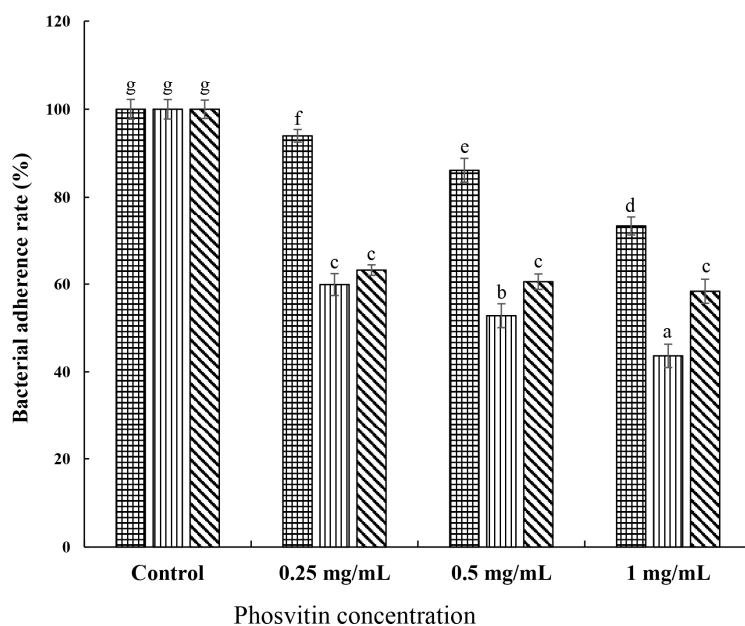
Fig. 3. Effects of phosvitin on adherence against Streptococcus mutans . ■, S. mutans KCTC 5124, ▨, S. mutans KCTC 5458, and ▩, S. mutans KCTC 5316. Values are expressed as the mean±SD. a-g Different letters among samples indicate significant differences (p<0.05). Control, non-treated group.
