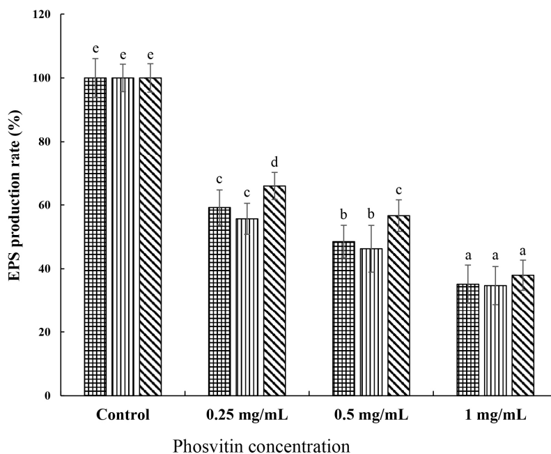
Fig. 4. Effects of phosvitin on EPS production against Streptococcus mutans . ■, S. mutans KCTC 5124, ▨, S. mutans KCTC 5458, and ▩, S. mutans KCTC 5316. Values are expressed as the mean±SD. a-e Different letters among samples indicate significant differences ( p < 0.05 ). Control, non-treated group; EPS, extracellular polysaccharides.
