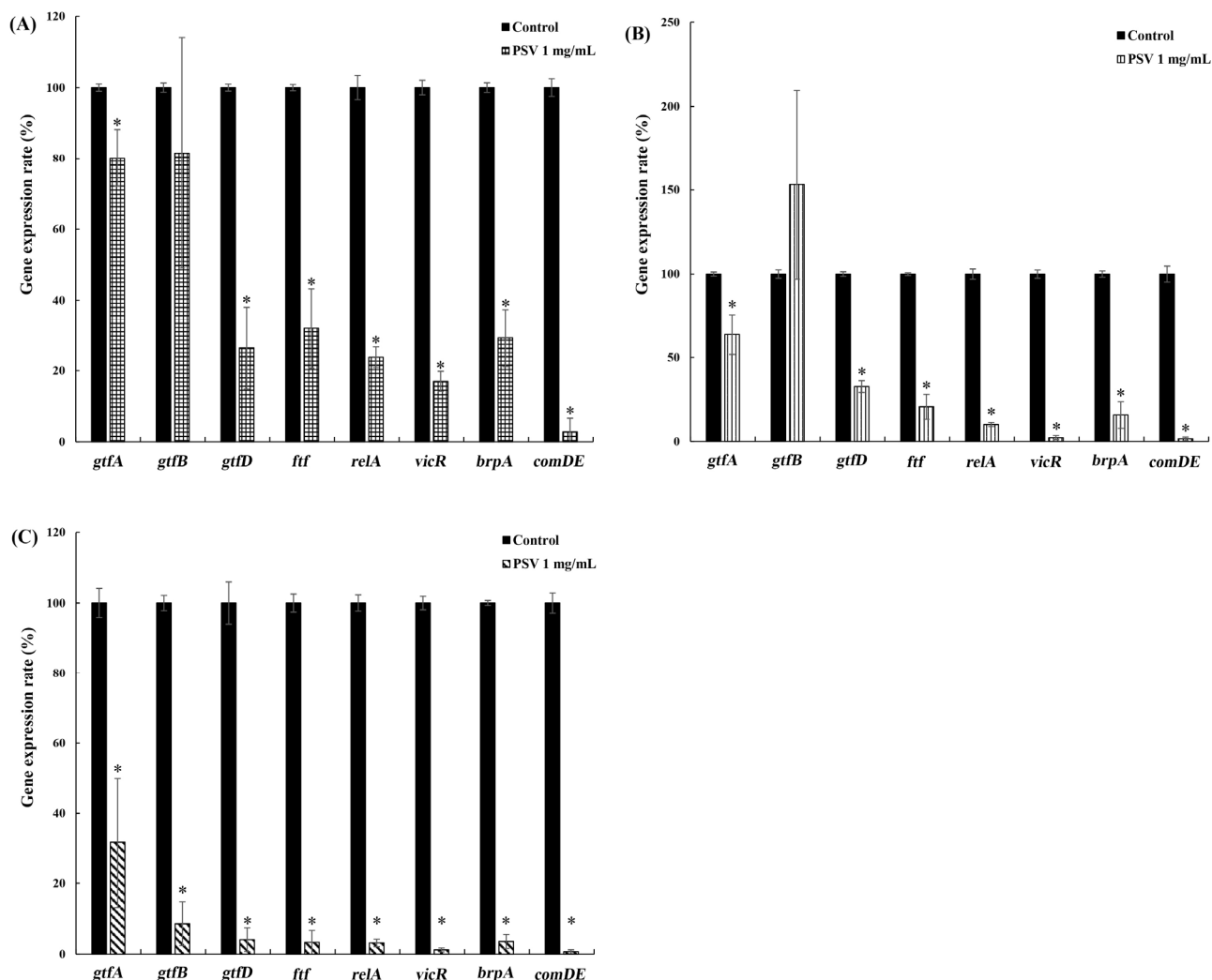
Fig. 5. Expression of virulence genes of Streptococcus mutans by qRT-PCR. (A) S. mutans KCTC 5124, (B) S. mutans KCTC 5458 and (C) S. mutans KCTC 5316. Values are expressed as the mean \pm SD and analyzed by student's t-test, with p < 0.05 considered as statistically significant. Control, non-treated group.
