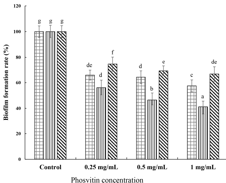
Fig. 1. Effects of phosvitin on biofilm formation against Streptococcus mutans . ■, S. mutans KCTC 5124, ▨, S. mutans KCTC 5458, and ▩, S. mutans KCTC 5316. Values are expressed as the mean±SD. a-g Different letters among samples indicate significant differences ( p < 0.05 ). Control, non-treated group.
