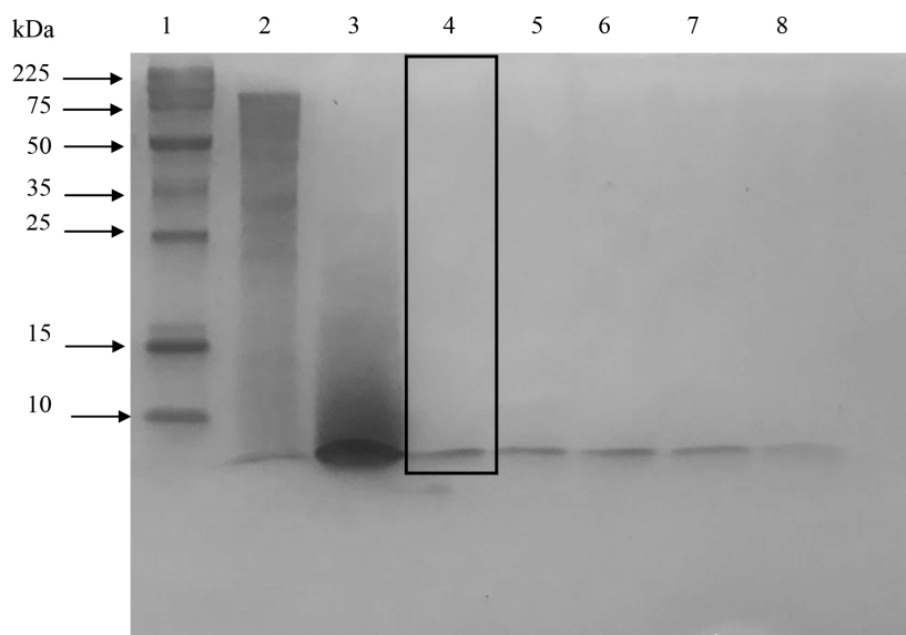
Fig. 1. The SDS-PAGE image of ovotransferrin hydrolyzed with protease; lane 1, marker; lane 2, ovotransferrin (1 mg/mL); lanes 3–8, ovotransferrin hydrolyzed with protease 55°C for 0, 3, 6, 9, 12, and 24 h. SDS-PAGE, sodium dodecyl sulfate-polyacrylamide gel electrophoresis.
