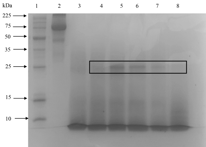
Fig. 2. The SDS-PAGE image of ovotransferrin hydrolyzed with papain; lane 1, marker; lane 2, ovotransferrin (1 mg/mL); lanes 3–8, ovotransferrin hydrolyzed with papain 37°C for 0, 3, 6, 9, 12, and 24 h. SDS-PAGE, sodium dodecyl sulfate-polyacrylamide gel electrophoresis.
