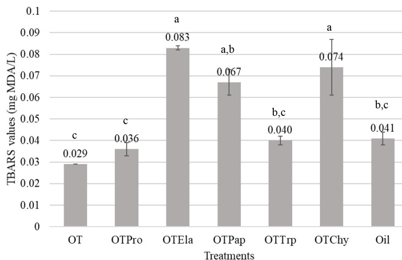
Fig. 4. Graphical illustration of TBARS value of oil emulsion (mg of malondialdehyde/L) of the ovotransferrin hydrolysates. Values with different letters are significantly different ( p < 0.05 ). TBARS, 2-thiobarbituric acid reactive substance.
