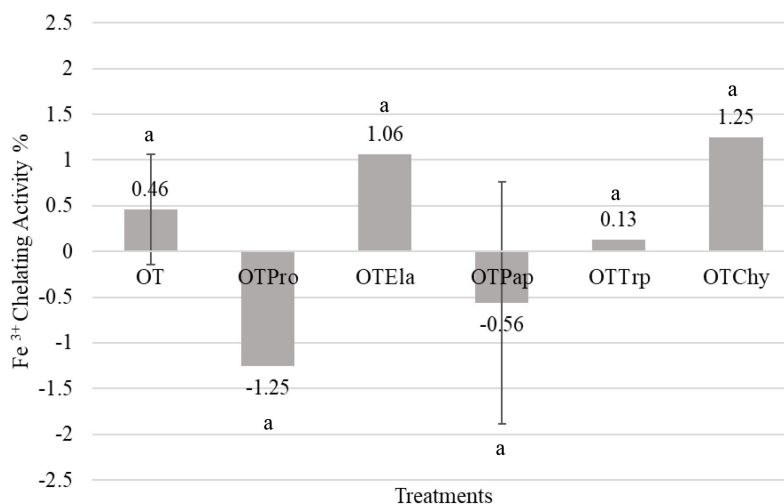
Fig. 5. Graphical illustration of Fe 3+ -chelating activity of the ovotransferrin hydrolysates. Values are mean with standard error. Values with different letters are significantly different ( p < 0.05 ).
