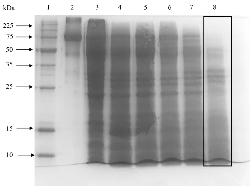
Fig. 3. The SDS-PAGE image of ovotransferrin hydrolyzed with elastase; lane 1, marker; lane 2, ovotransferrin (1 mg/mL); lanes 3–8, ovotransferrin hydrolyzed with elastase 25°C for 0, 3, 6, 9, 12, and 24 h. SDS-PAGE, sodium dodecyl sulfate-polyacrylamide gel electrophoresis.
