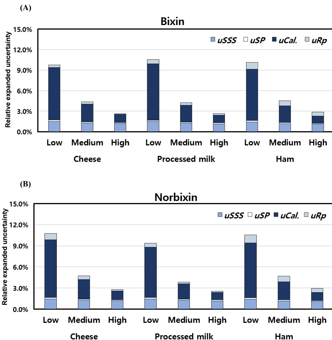
Fig. 2. Contributions of measurement uncertainty to the relative expanded uncertainty of Bixin and Norbixin spiked in cheese, processed milk, and ham. Bixin (A), Norbixin (B). uSSS , uncertainty of standard stock solution; uSP , uncertainty of sample preparation; uCal. , uncertainty of the calibration of standard; uRp , uncertainty of repeatability.
